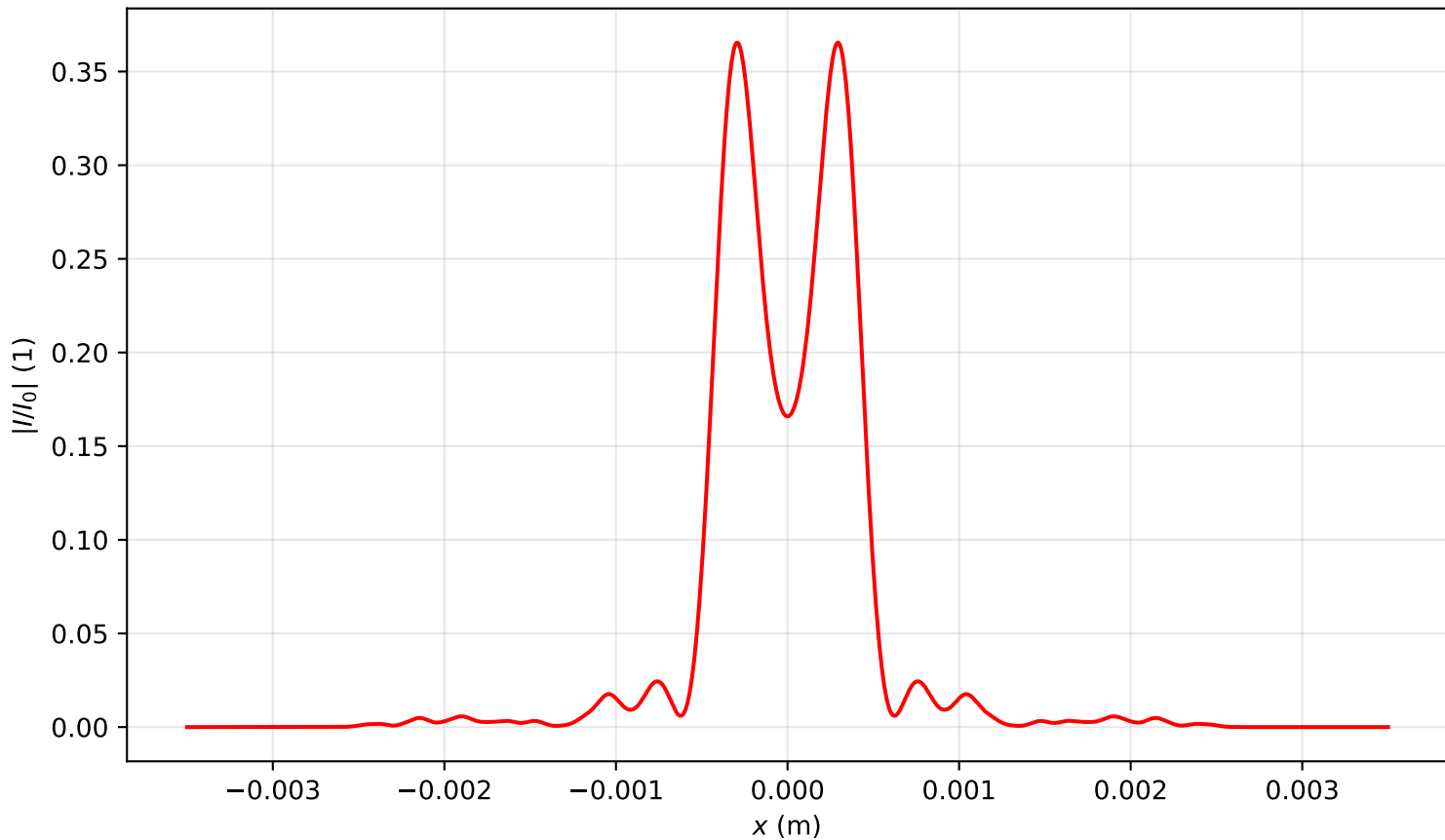
Intensity profile I(x, y = 0, z = 1.592)/I_0 , P_{in}=4.0P_{cr} , artificial time
